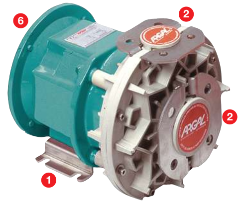
Integral version (only plastic), sealed, close-coupled execution.
